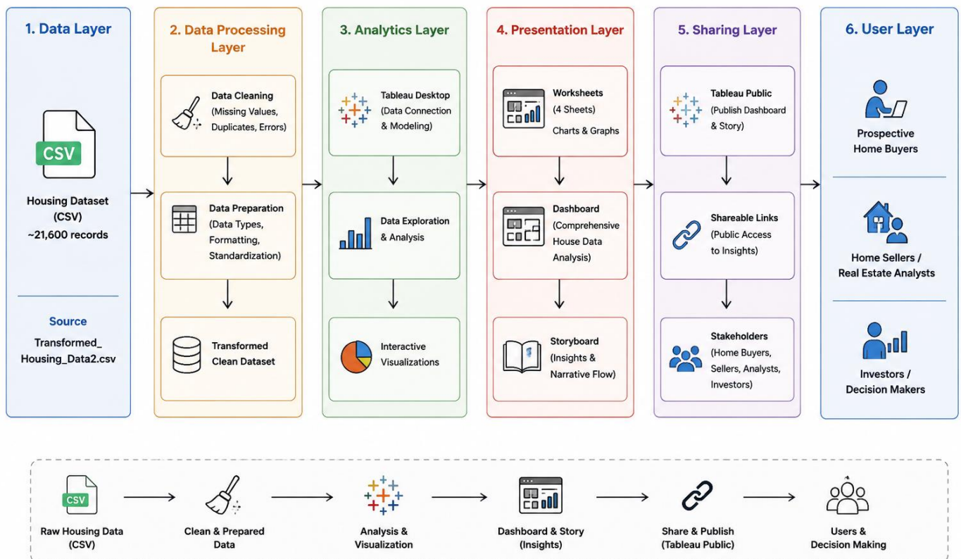
Figure: Architecture and data flow of the Housing Market Trends Tableau dashboard
